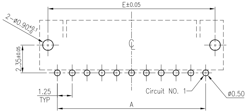
PCB. LAYOUT
